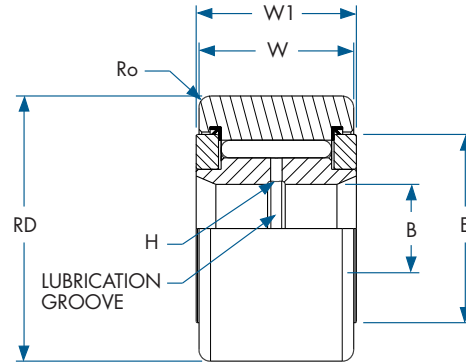
CAM YOKE ROLLER CYLINDRICAL (CCYR)
