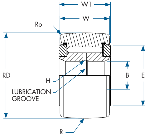
CAM YOKE ROLLER SPHERICAL (CYR)
